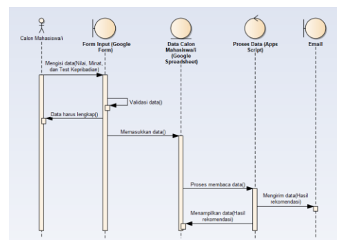
Gambar 2. Sequence Diagram
