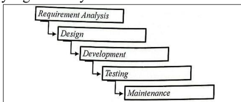
Gambar 1. Metode Waterfall
